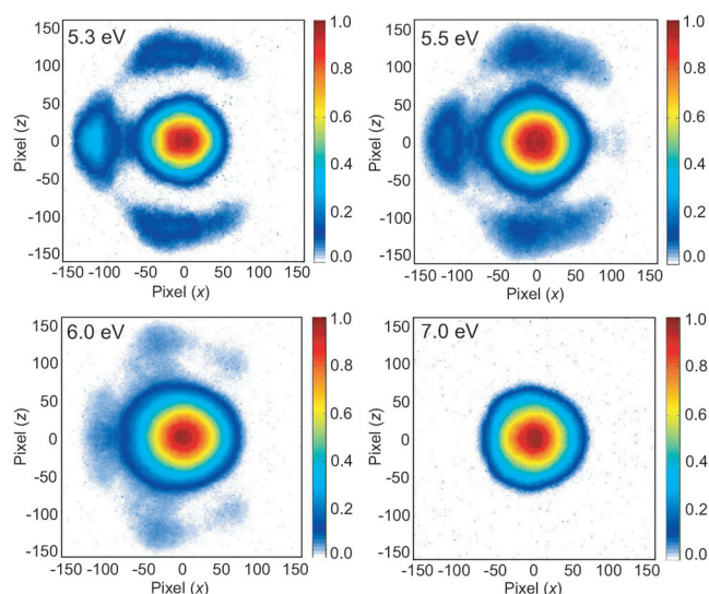
Figure 1. Slice images of F^- recorded at 5.3, 5.5, 6.0, and 7.0 eV. The intensities are normalized and the electron incident direction is from left to right.
