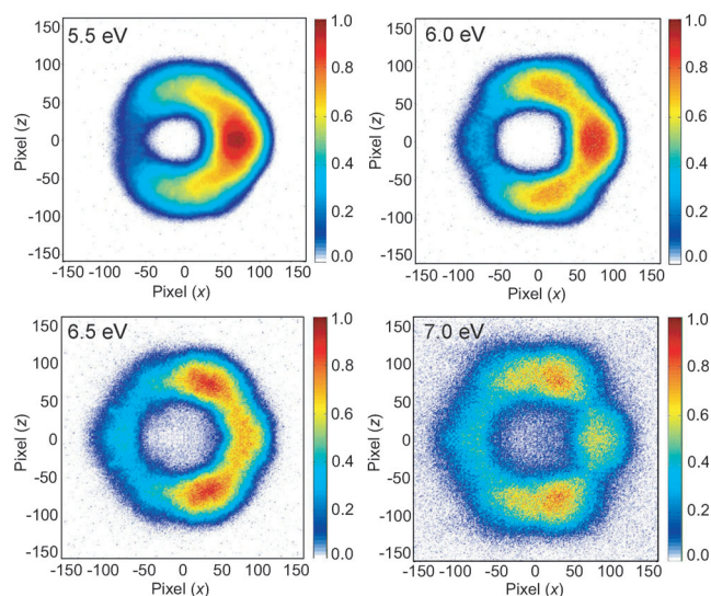
Figure 2. Slice images of CF_3^- recorded at 5.5, 6.0, 6.5, and 7.0 eV. The intensities are normalized and the electron incident direction is from left to right.
