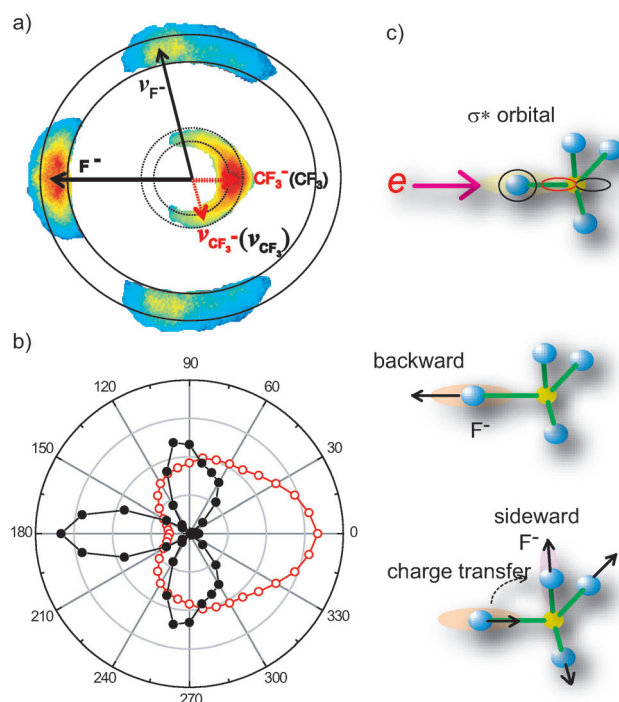
Figure 3. a) The kinetic correlation between the faster F^- and CF_3^- fragments: here v(CF_3) = v(CF_3^-) in which CF_3 is the product of CF_4^- \rightarrow F^- + CF_3 ; two annular areas (recorded at the electron energy of 5.5 eV and with intensity renormalizations) correspond to the kinetic energies of 0.90–1.60 eV ( F^- ) and 0.25–0.45 eV ( CF_3^- ). b) The angular distributions of F^- (solid circles), CF_3^- (empty circles), and the ion intensities are obtained with integrations of the ion signals in the above-mentioned two annular areas and normalized. c) The orientation effect on the F^- momentum distributions.
